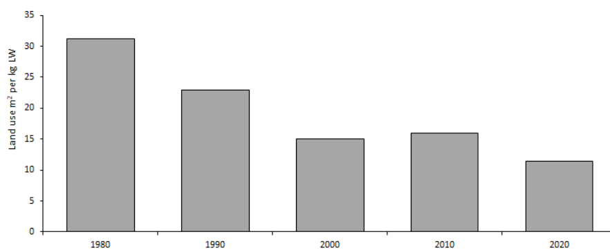
Figure 6 Changes in land use from the production of 1 kg live weight pork over the period 1980 to 2020
