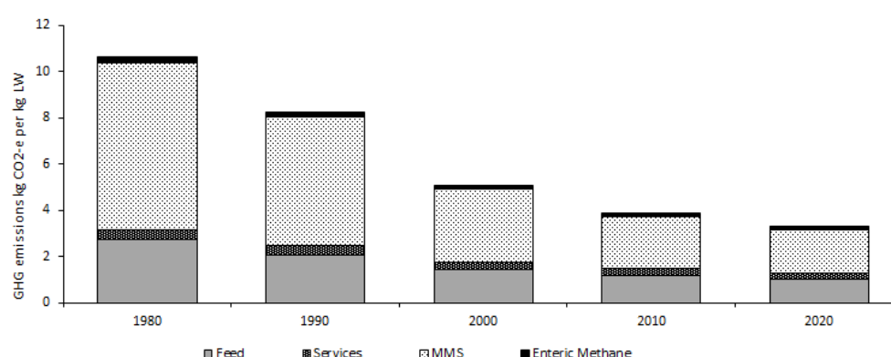
Figure 3 Changes in greenhouse gases emissions (excluding LU and dLUC) from the production of 1 kg of live weight pork over the period 1980 to 2020
