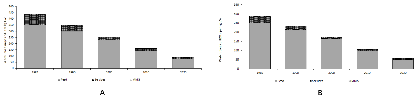
Figure 5 Changes in water consumption (A) and water stress (B) from the production of 1kg live weight pork over the period 1980 to 2020
